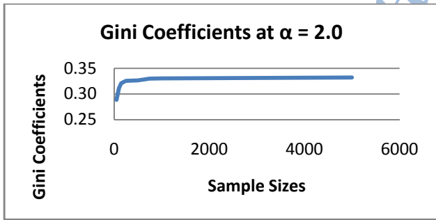
Figure 3: Line Graph of Gini coefficients when \alpha=2.0
