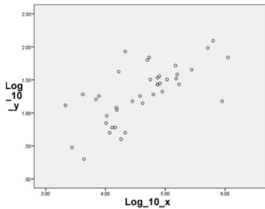
Figure 3b: Graph of \text{Log}_{10}y against \text{Log}_{10}x (transformed data)
