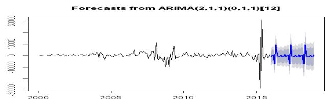
Figure 8: Forecasts from SARIMA (2,1,1)x(0,1,1) 12
