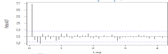
Figure 3: Sample PACF of NSE ASI Series
