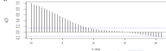
Figure 2: Sample ACF of NSE ASI Series
