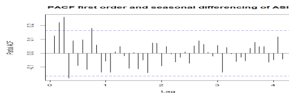
Figure 6: Sample PACF of First Order and Seasonal Differencing of ASI
