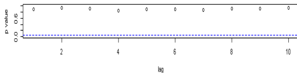
Figure 7: Adequacy Check For Sarima(2,1,1)X(0,1,1) 12 using ACF of Residuals
