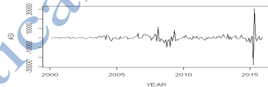
Figure 4: Plot of the first and seasonal differences of NSE ASI Series
