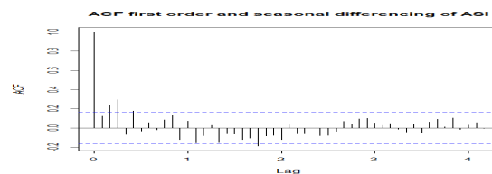
Figure 4: Plot of the first and seasonal differences of NSE ASI Series
